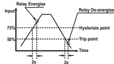
4) Lo alarm & De-energised relay
