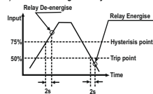
3) Lo alarm & Energised relay
